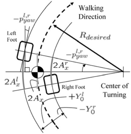
Fig. 7. Foot prints captured in double support phase during a turning walk. Step length and leg yaw rotation are modulated with respect to a desired circular radius, R_{desired} . We assume that the origin of body-fixed coordinates moves along the desired circular arc (dashed arc). We use 2A_x to denote the step length for a straight walk and 2A_x^l , 2A_x^r are modulated step lengths in order to satisfy kinematic constraints without slippage due to lateral leg position offset Y_0^l , Y_0^r , respectively. Here -p_{yaw}^{l,r} indicates the angle of necessary yaw rotation.
